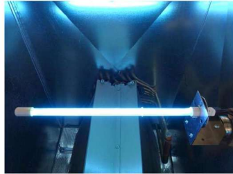
Low voltage 24VAC ballast w/ Lamp and Ballast Monitoring Electronics
